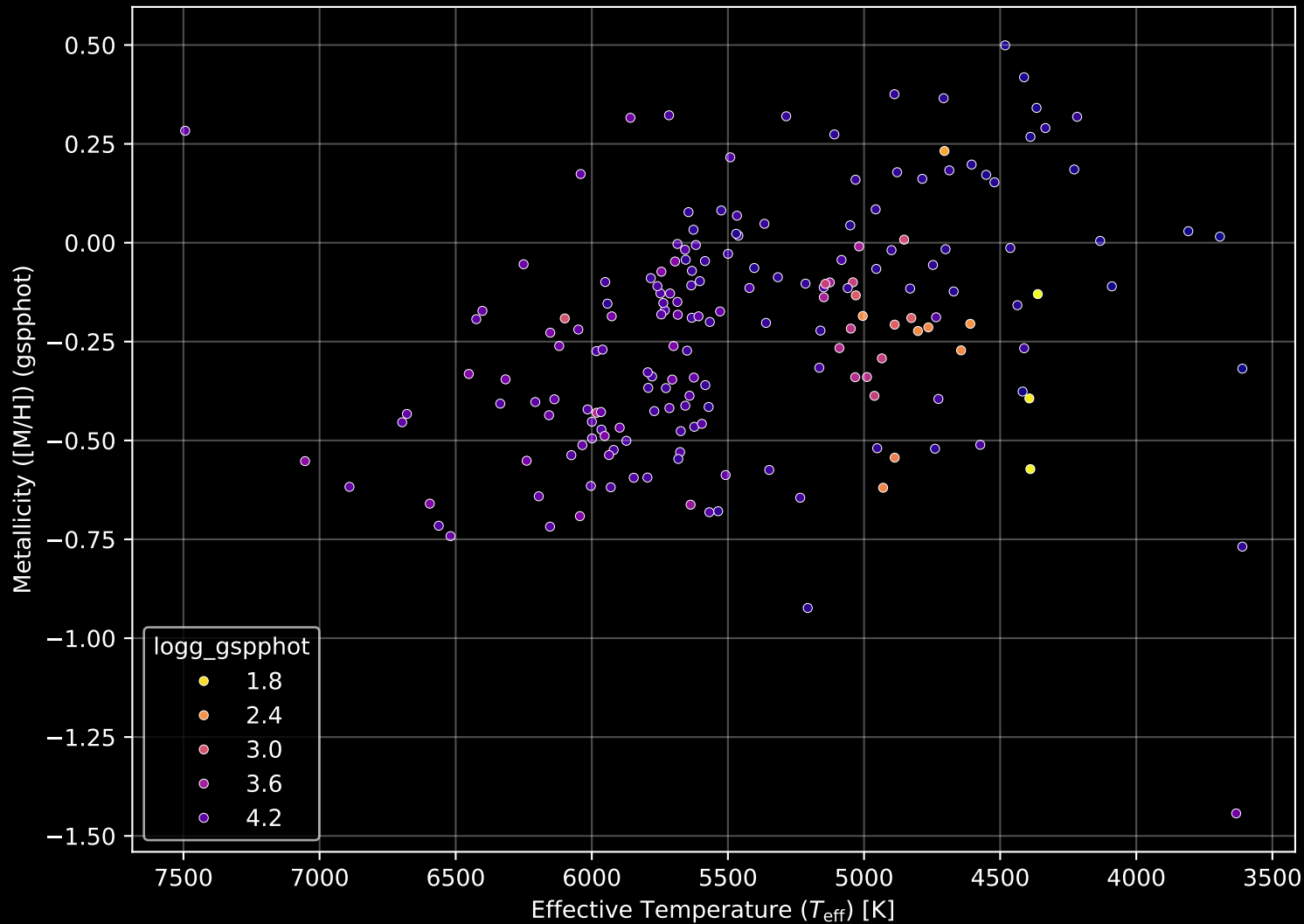
APOGEE DR17 Field: [100+70_MGA] Stellar Population Parameters (n= 186)
