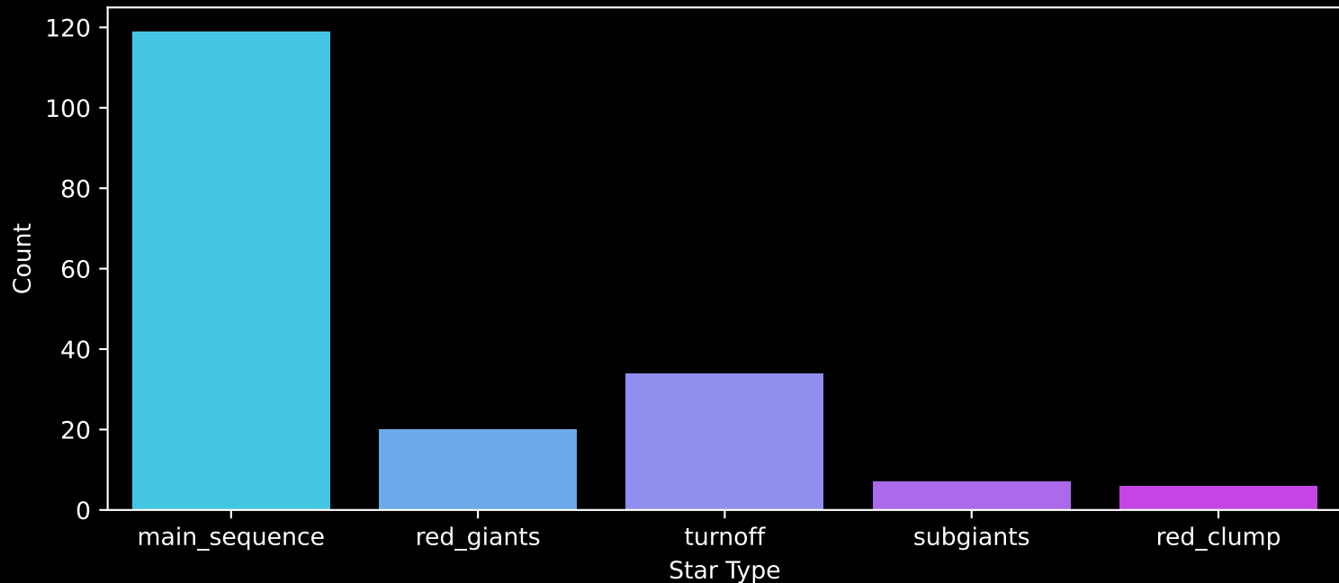
APOGEE DR17 Field: [100+70_MGA] Count plot of Star Type
