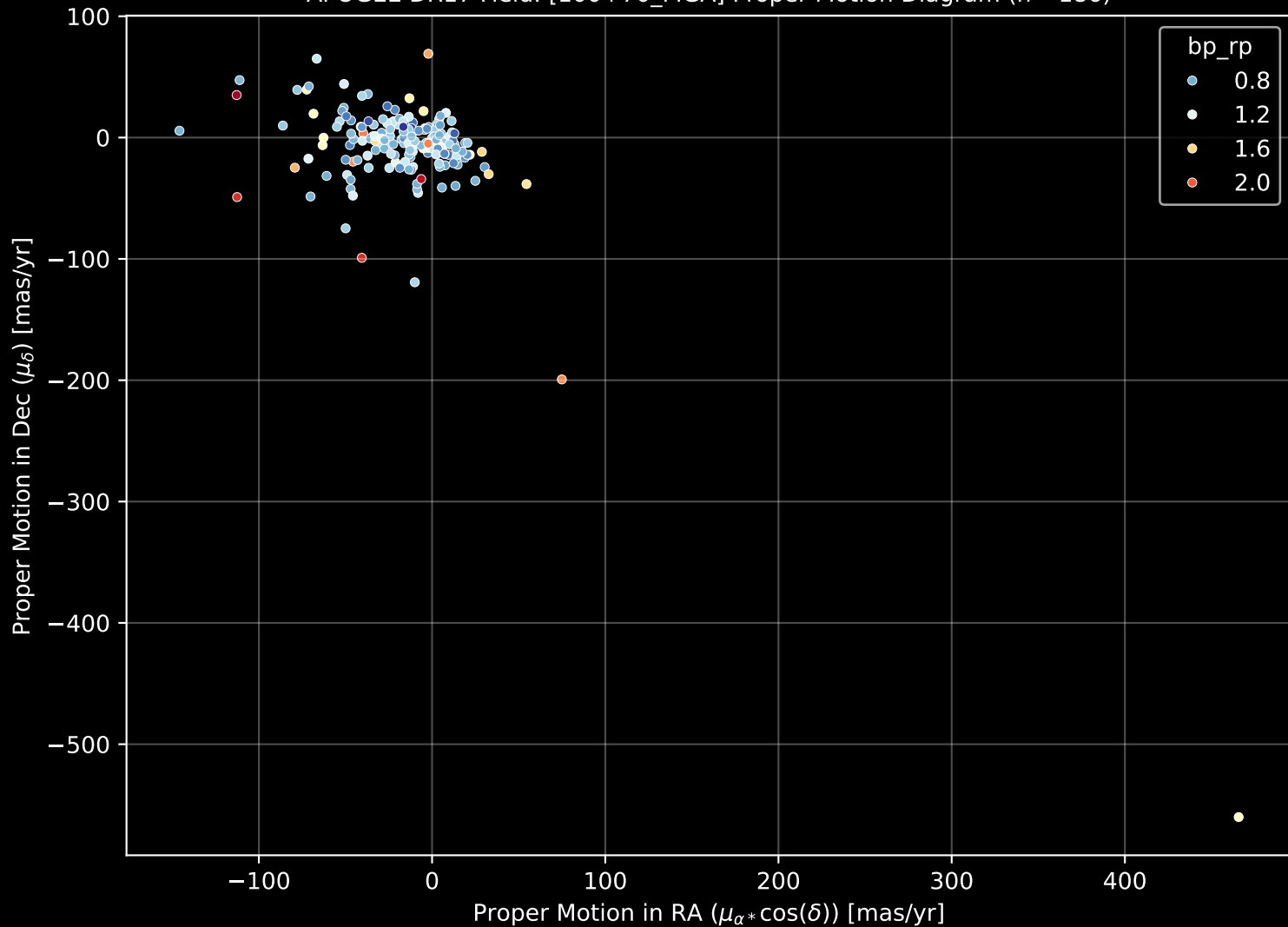
APOGEE DR17 Field: [100+70_MGA] Proper Motion Diagram (n= 186)
