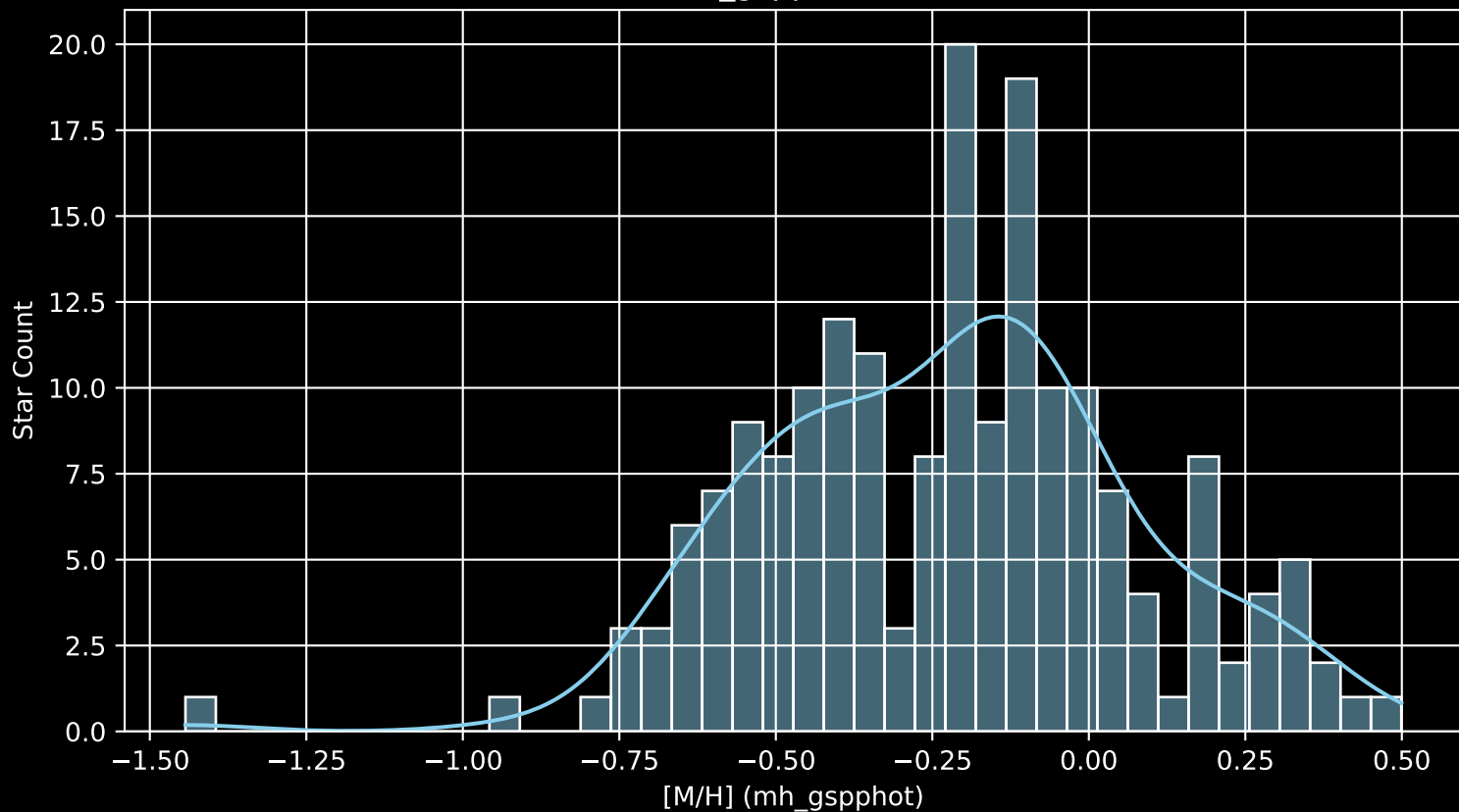
APOGEE DR17 Field: [100+70_MGA [M/H] (mh_gspphot) (n= 186)
