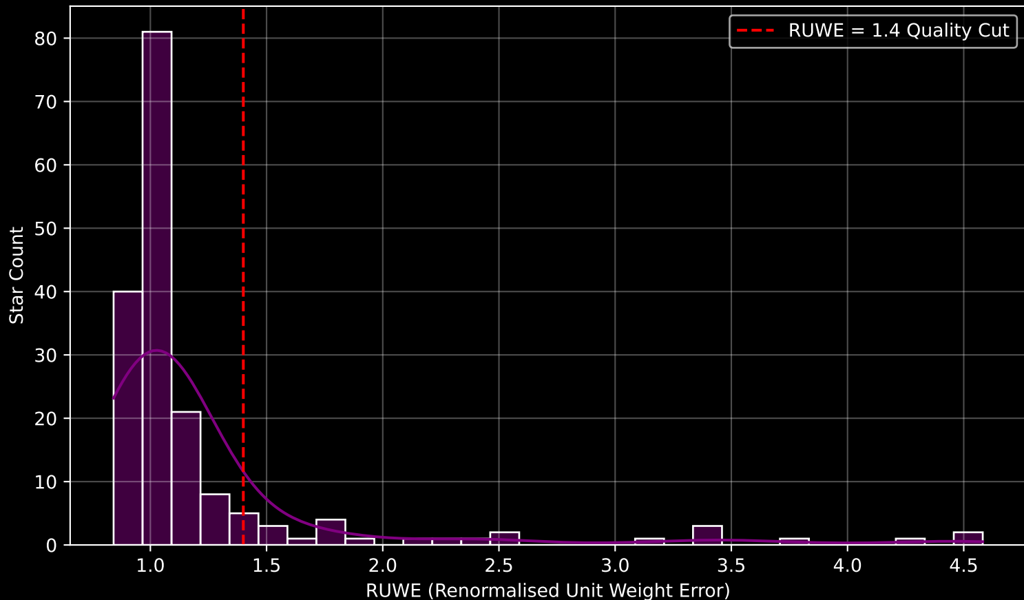
GAPOGEE DR17 Field [100+70_MGA] RUWE Distribution (n= 177)
