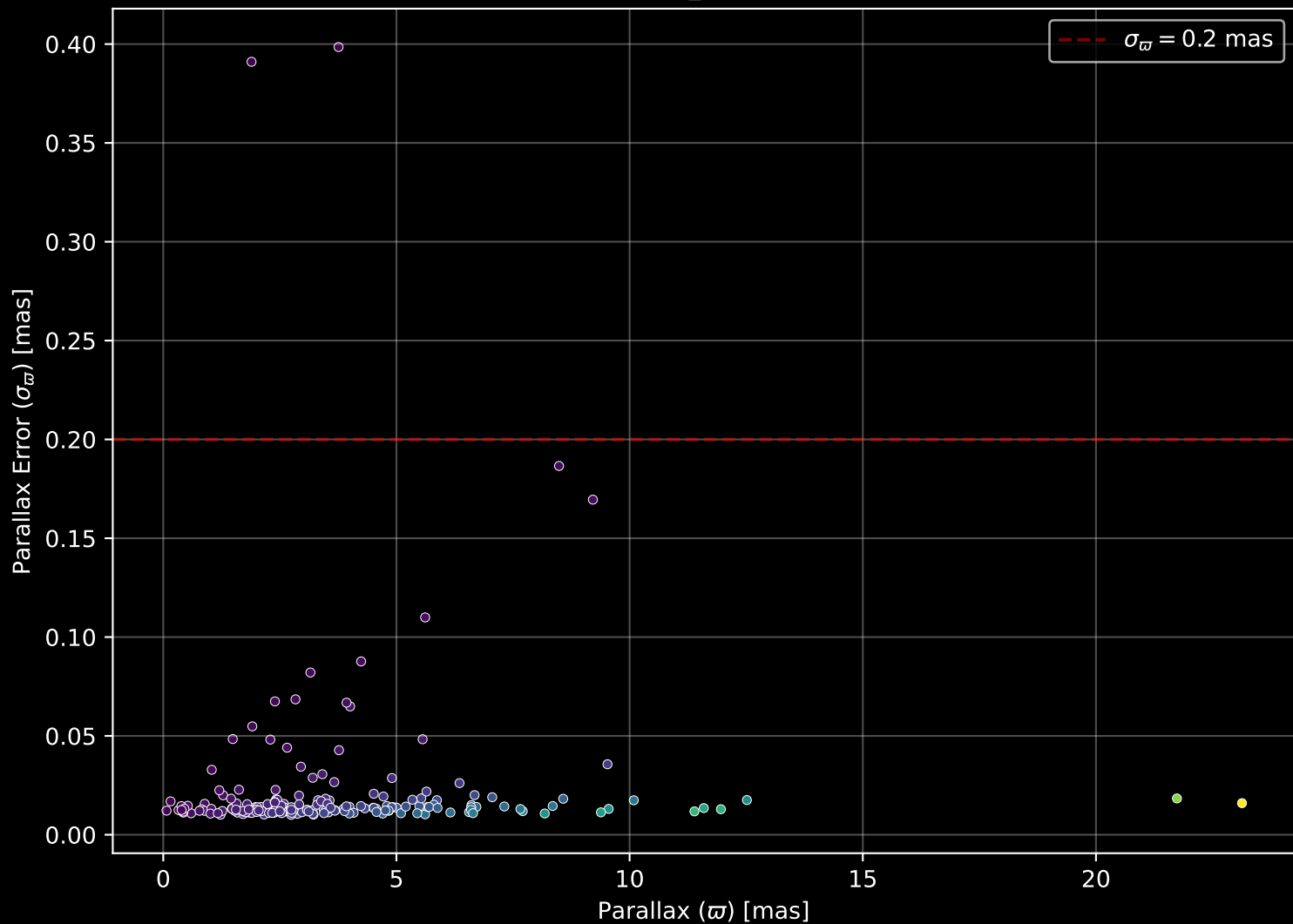
APOGEE DR17 Field: [100+70_MGA] Parallax Quality (n= 186)
